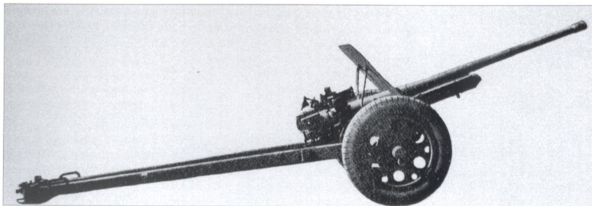
The Japanese 47mm Type 1 (1941) AT gun. The Japanese were extremely proficient in positioning these and other weapons in well camouflaged positions to achieve flank and rear shots at the US Shermans during the late war island battles, and under such circumstances they did achieve 'kills' despite their mediocre performance.
